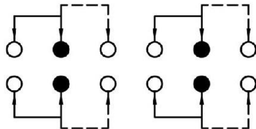
SCHEMATIC (SHORTING)
